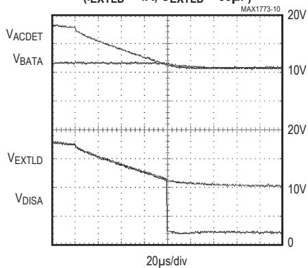
TRANSITION FROM AC ADAPTER TO BATTERY A (I EXTLD = 4A, C EXTLD = 66μF)
