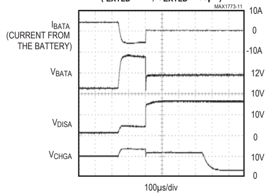
TRANSITION FROM BATTERY A TO AC ADAPTER (I EXTLD = 4A, C EXTLD = 66μF)
