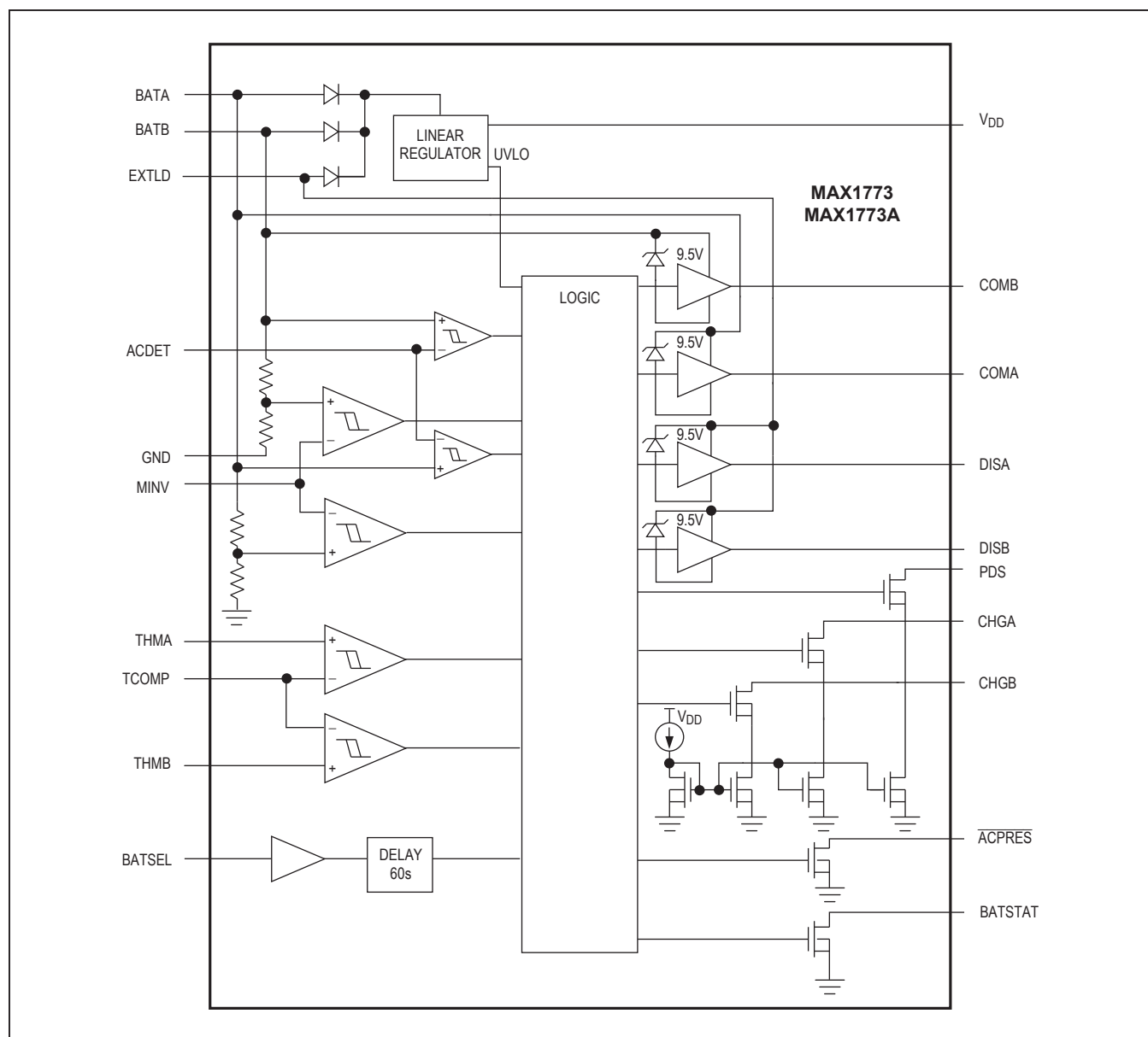
Figure 11. Functional Diagram
