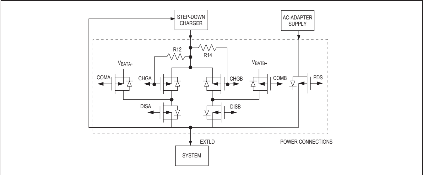
Figure 9. 7-MOSFET Topology
