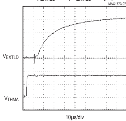
TRANSITION FROM BATTERY A TO BATTERY B (T COMP ) (I EXTLD = 4A, C EXTLD = 66μF)
