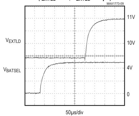
TRANSITION FROM BATTERY A TO BATTERY B (BATSEL) (I EXTLD = 4A, C EXTLD = 66μF)
