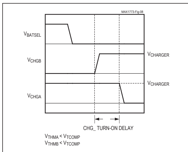
Figure 8. Charge Turn-On Delay (Battery B to Battery A)
