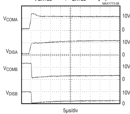
TRANSITION FROM BATTERY A TO BATTERY B (T COMP ) (I EXTLD = 4A, C EXTLD = 66μF)
