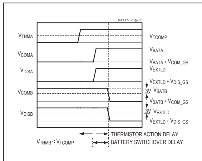
Figure 3. Thermistor Switchover Delay (Battery A to Battery B)
