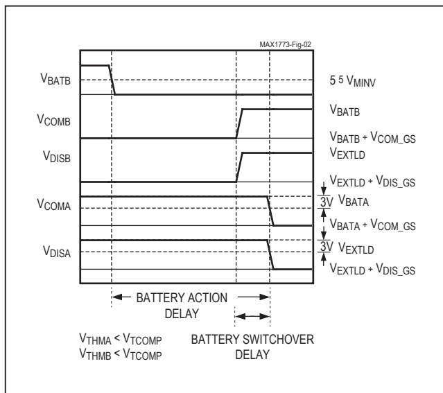
Figure 2. Battery Delay (Battery B to Battery A)
