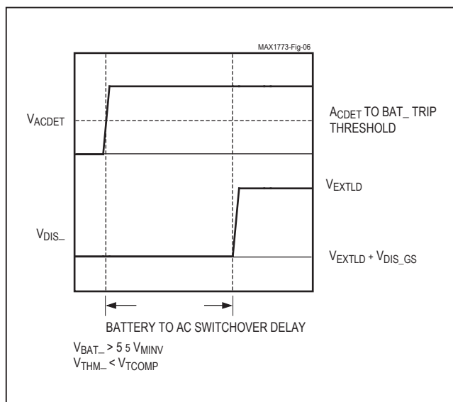
Figure 6. Battery to AC Switchover Delay
