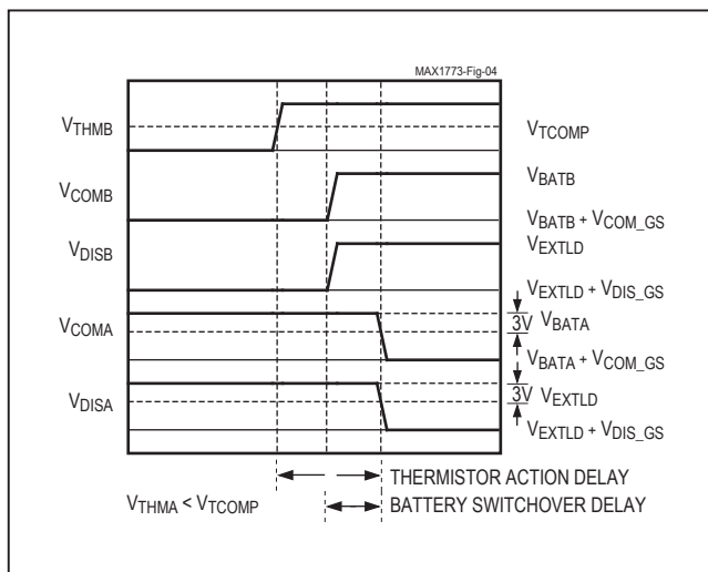
Figure 4. Thermistor Switchover Delay (Battery B to Battery A)
